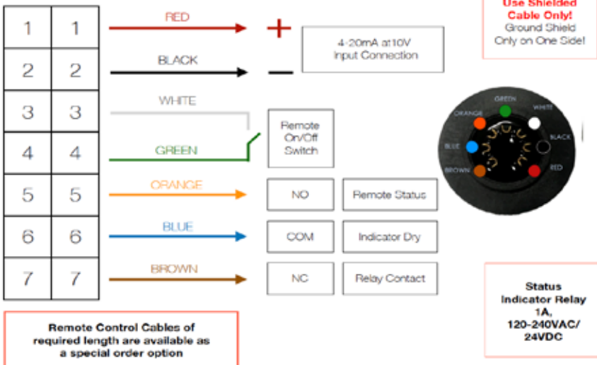
Standard Remote Control Schematic
